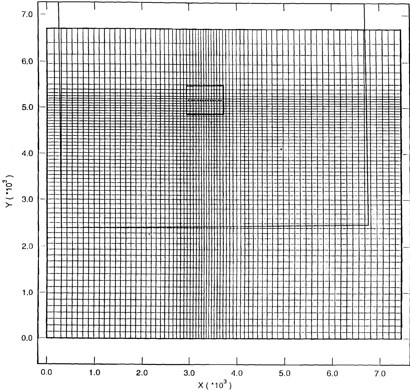
Figure APNS 7B.1 Locations (dots) of origins used in Particle Tracking Analyses
