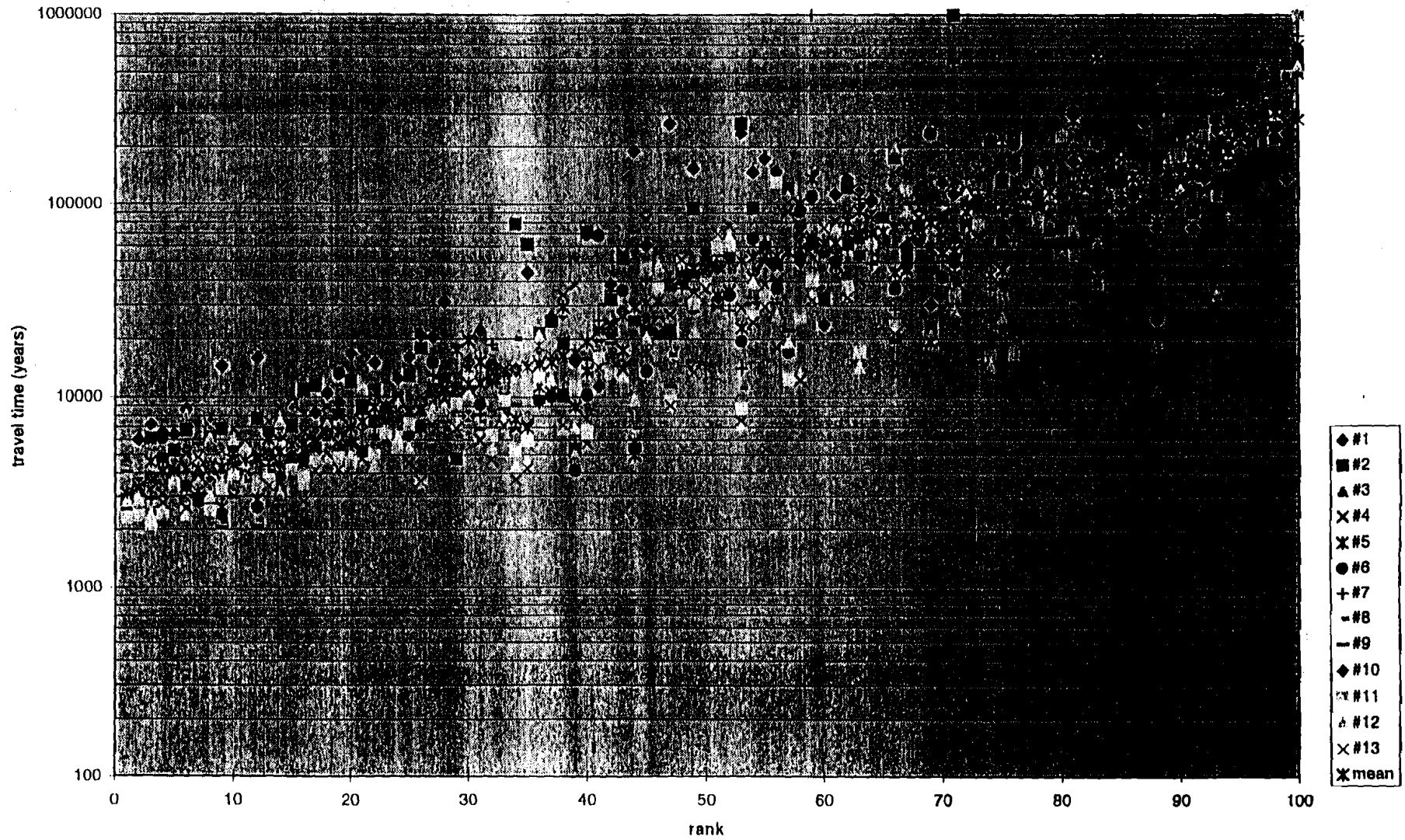
Figure NS7b.2 Scatter Plot of Travel Times: Full Mining Case (no Interconnections)
